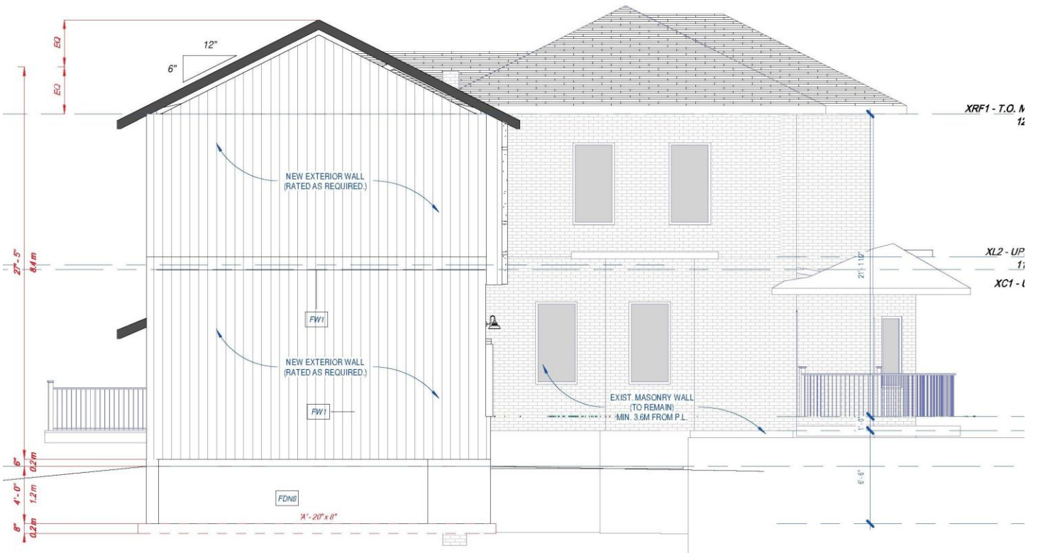
1 EAST ELEVATION 3/16" = 1'-0"
