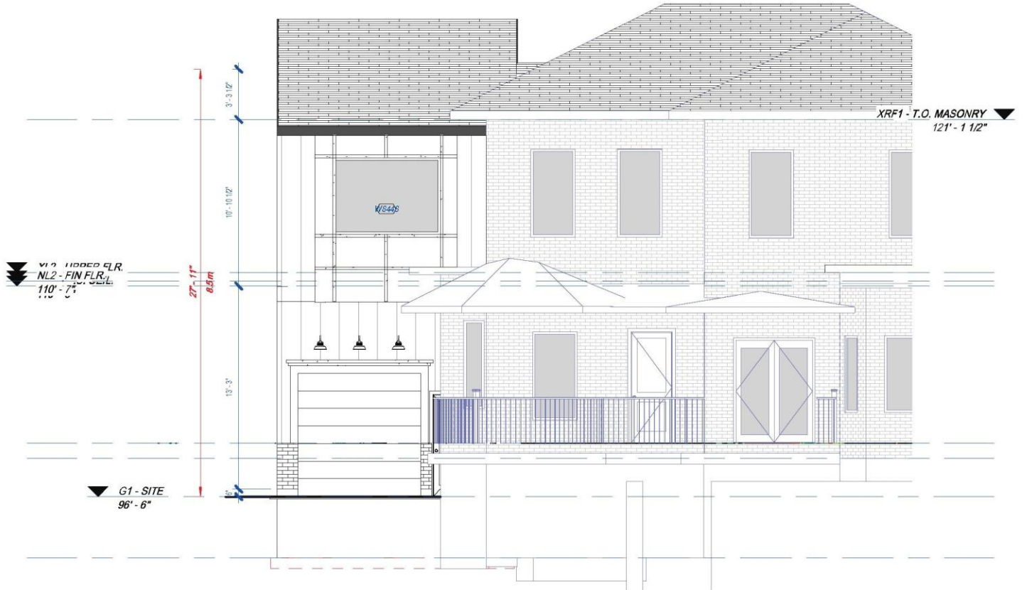
1 NORTH ELEVATION 3/16" = 1'-0"
